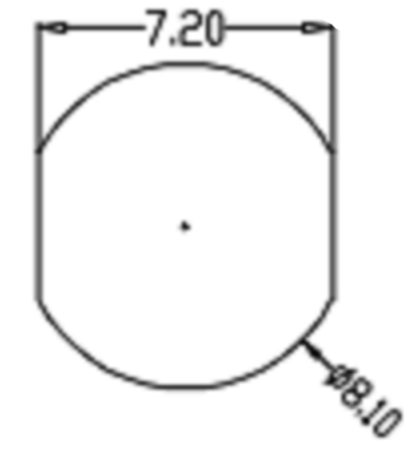
Recommended Panel Cut-out
