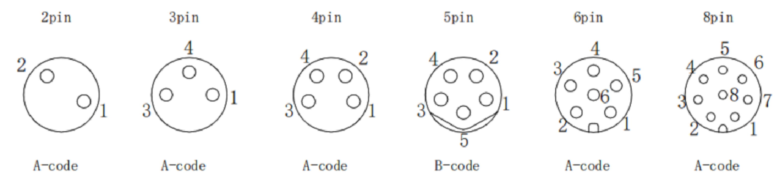
Pin assignment front view/针位分布前视图
